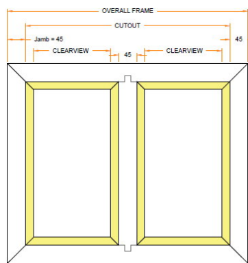
Double Pane
