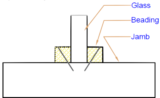
Square bead, glass centered
