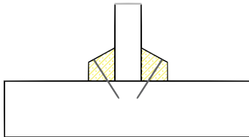
Bevel bead, glass centered
