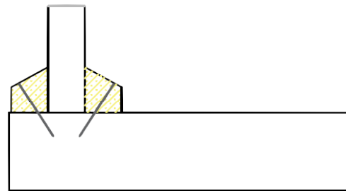
Bevel bead, glass to front
