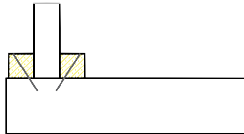
Square bead, glass to front
