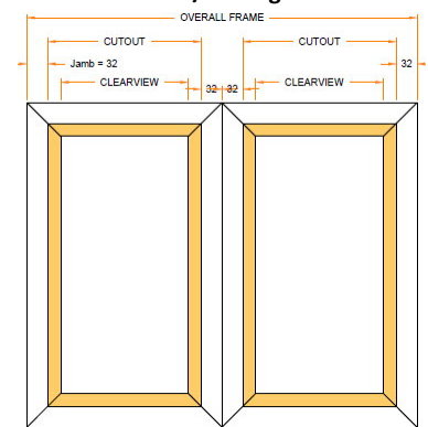
Joined Window / Sidelight
